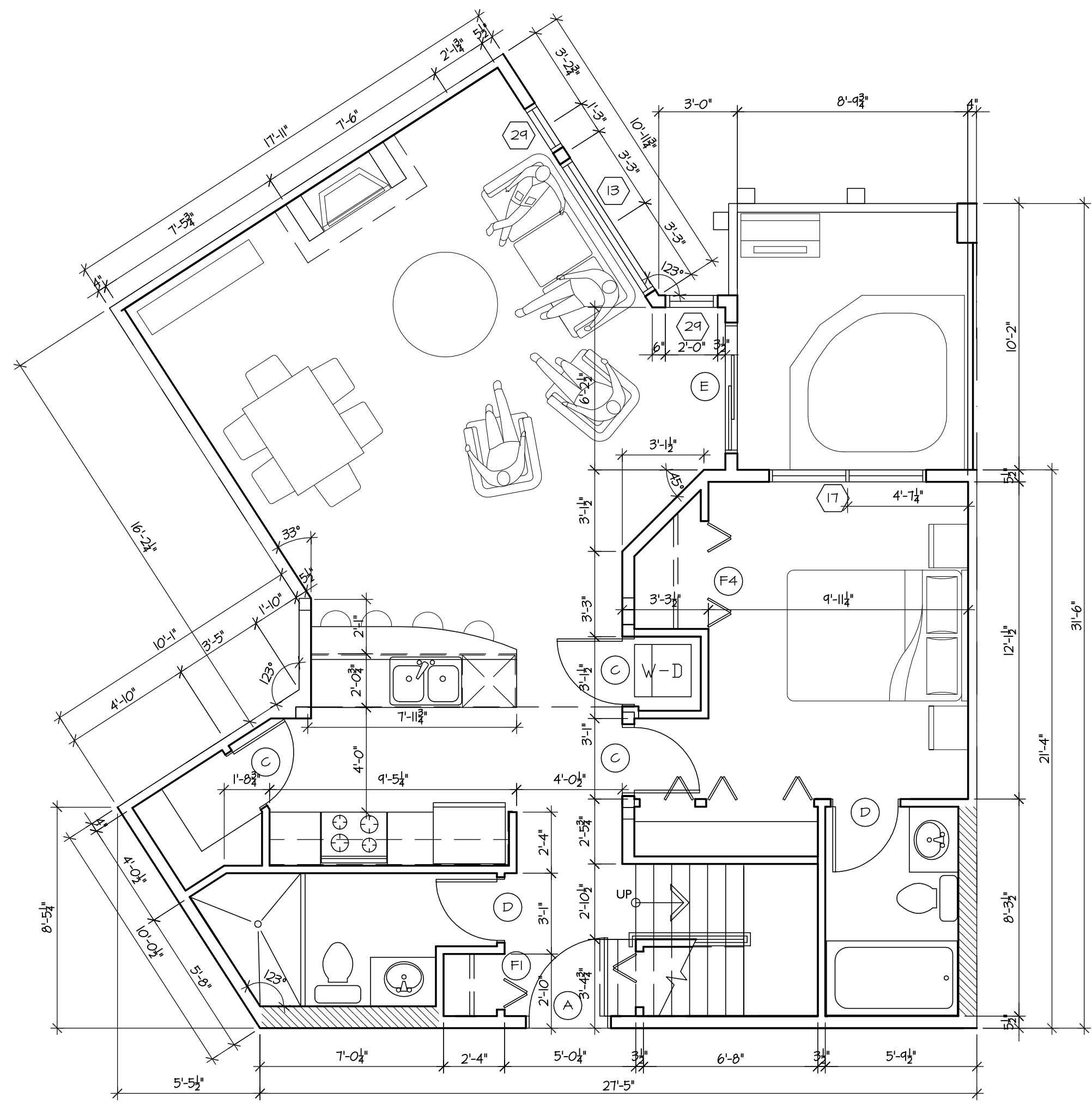
UNIT DL 1 BED & DEN - LOWER LEVEL 853 Sq Ft TOTAL - 853 + 187 = 1040 SQ.FT
